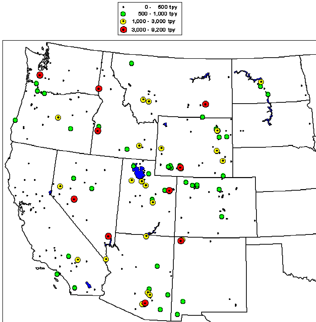
Figure II-2. Stationary PM 10 Emissions > 100 tpy in the WRAP Region (1996).
